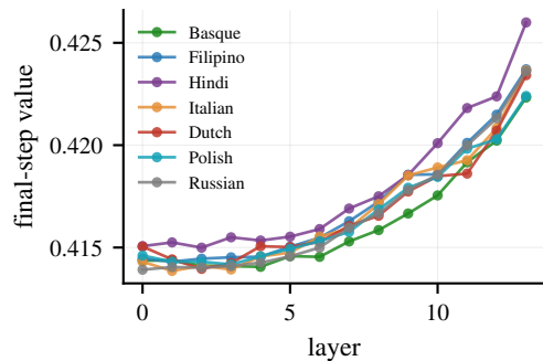
\kappa(W_{OV})
