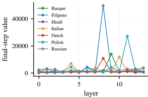
\kappa(W_{OV})
